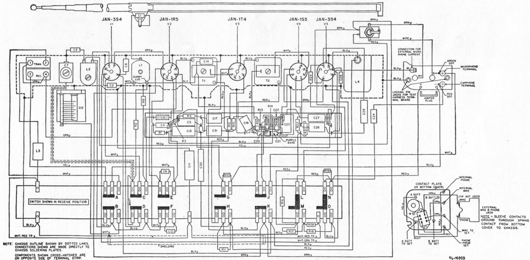
Figure 93. Radio Receiver and Transmitter BC-611-F, wiring diagram.
