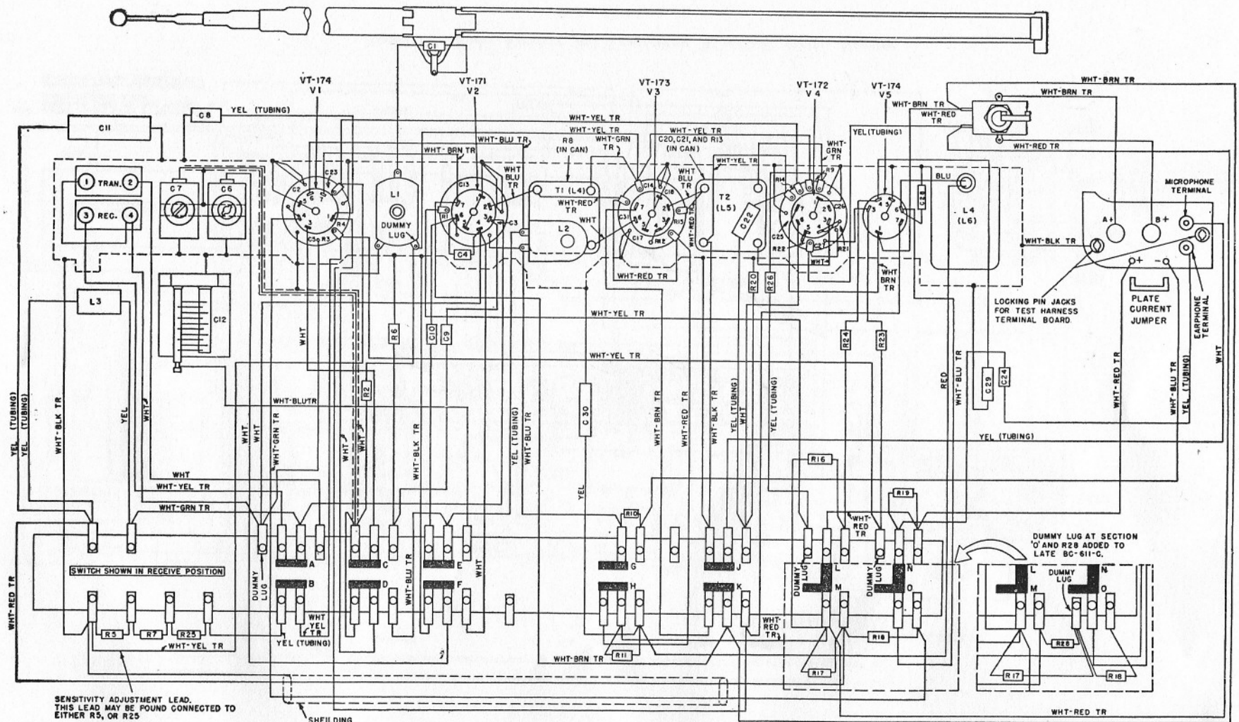
Figure 92. Radio Receiver and Transmitters BC-611-B through -E, wiring diagram.
