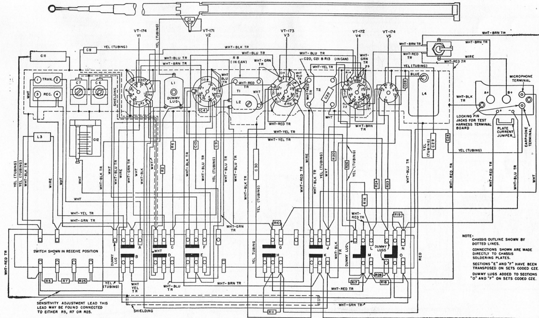
Figure 91. Sets coded CZE, wiring diagram.
