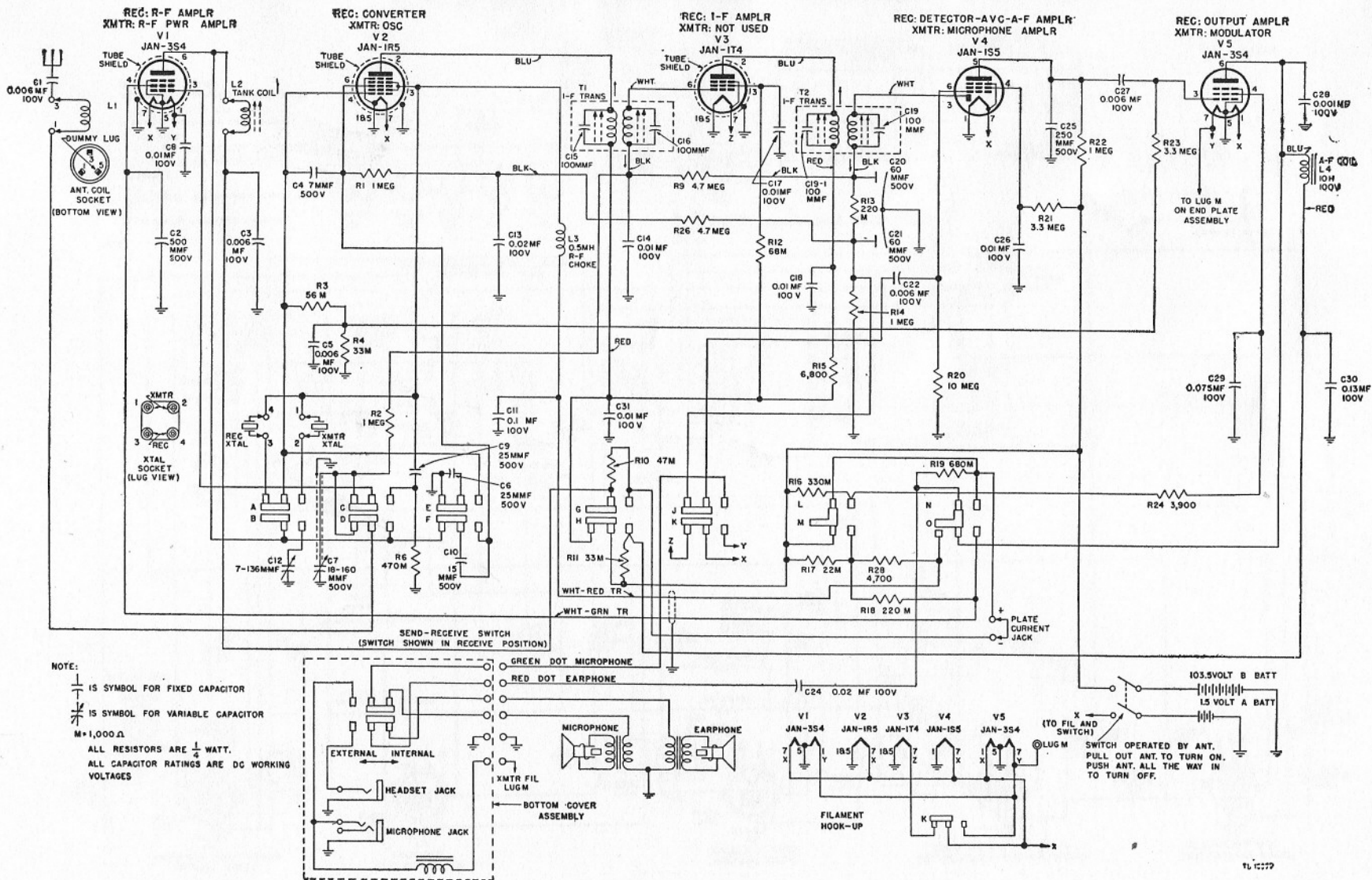
Figure 55. Radio Set SCR-536-F, complete schematic diagram.
