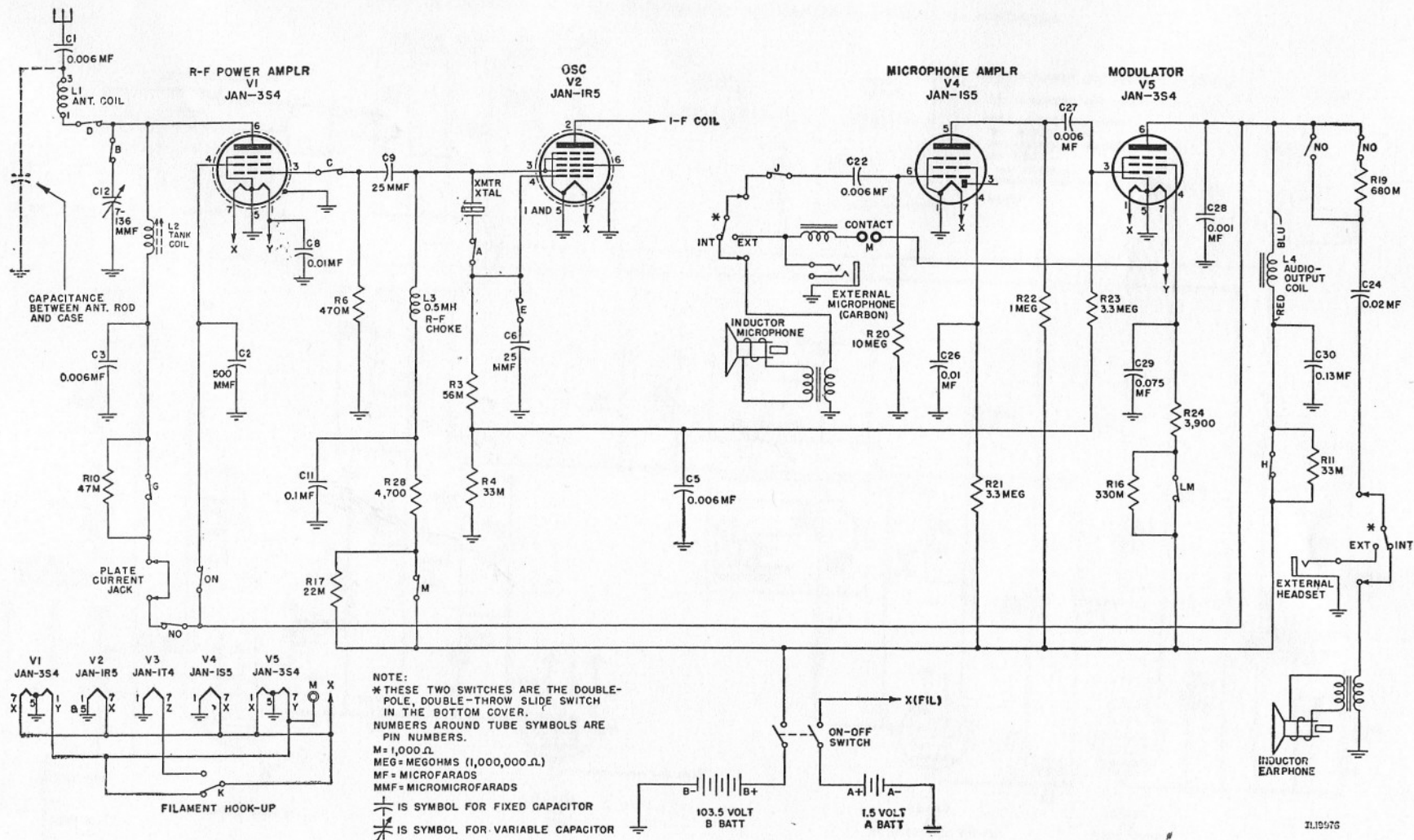
Figure 53. Radio Set SCR-536-F, functional diagram of transmitter.
