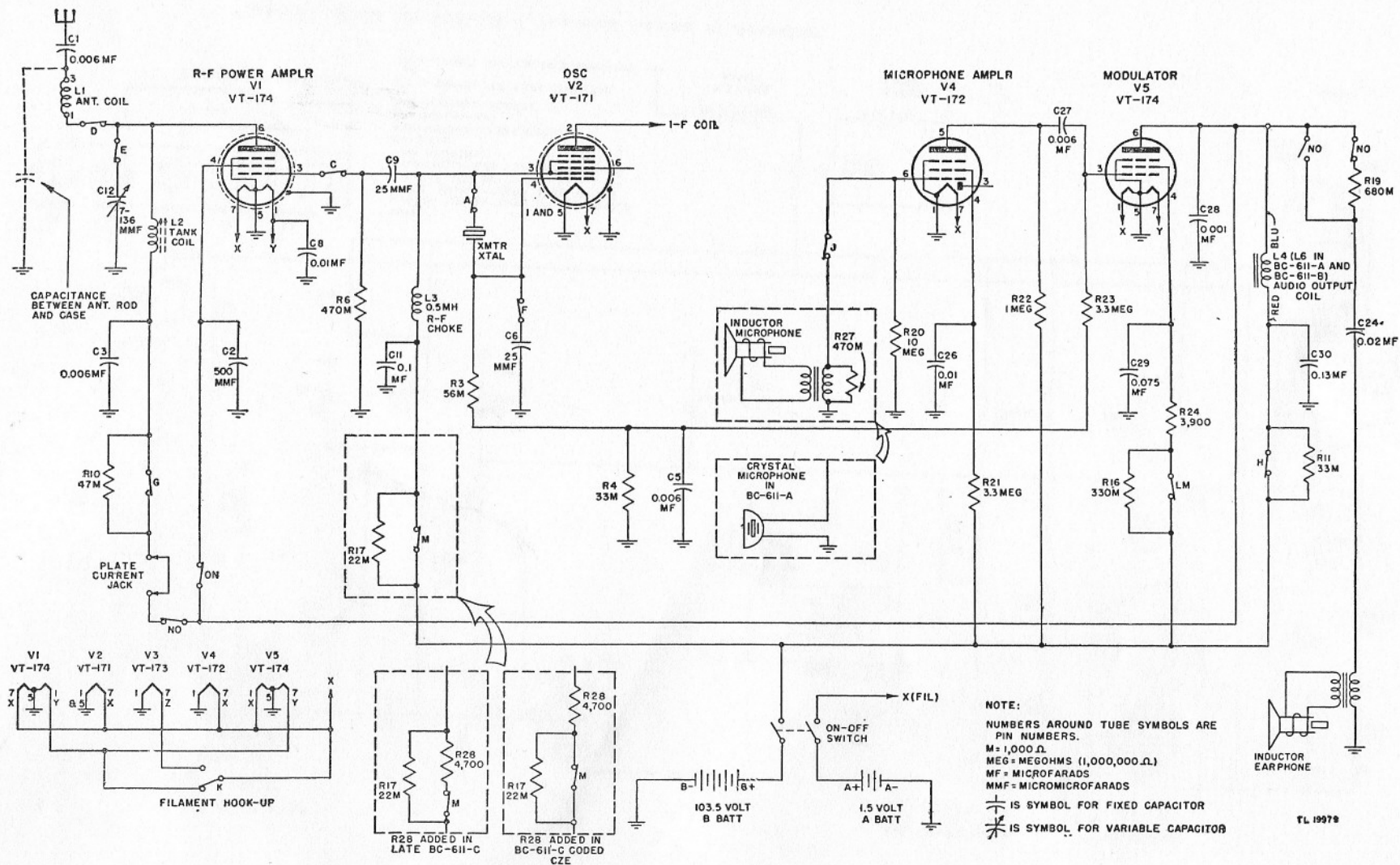
Figure 52. Radio Sets SCR-536-A through -E, functional diagram of transmitter.
