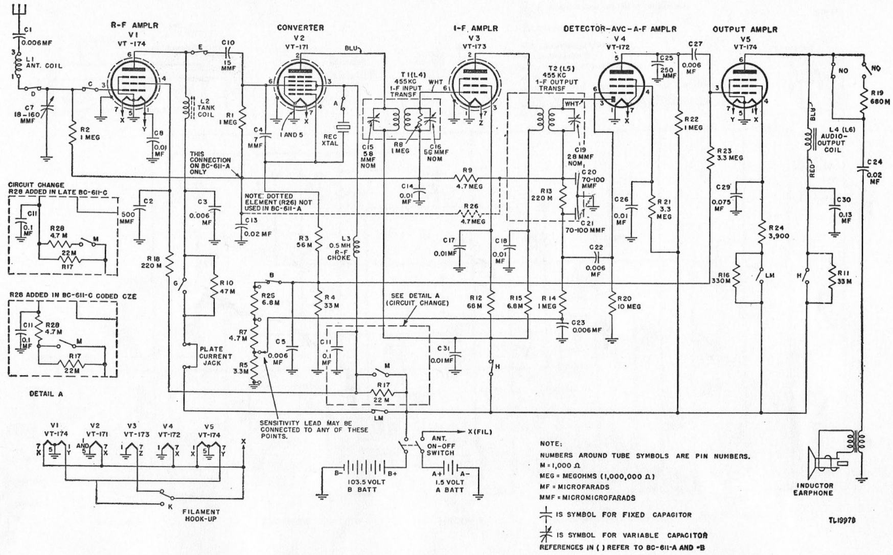
Figure 50. Radio Sets SCR-536-A through -E, functional diagram of receiver.
